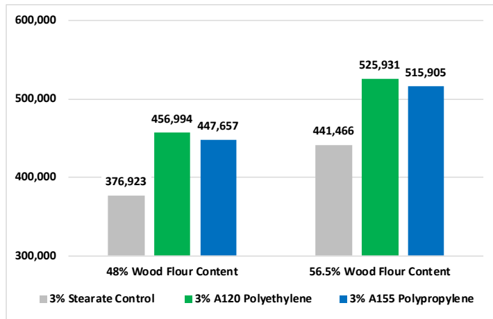
Chart 2: Modulus of Elasticity (PSI), ASTM D790
